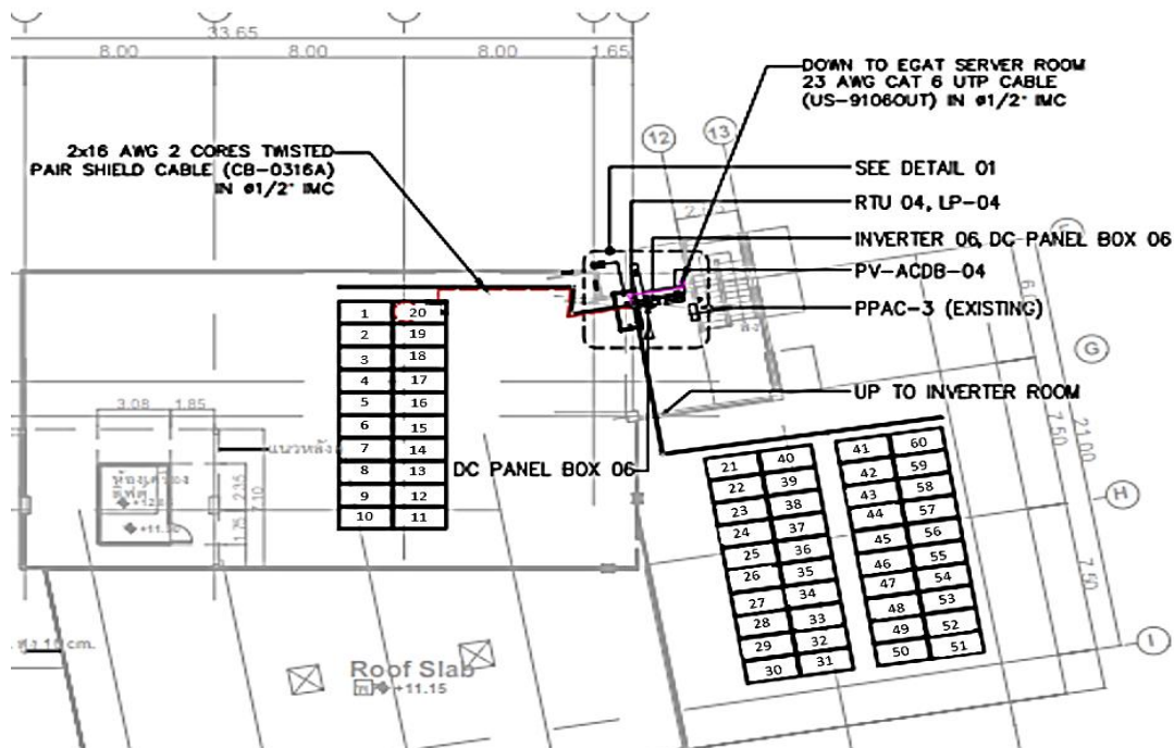
Layout T0020
