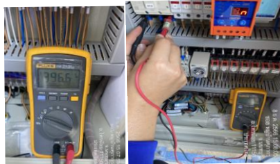
Voltage check1-3
